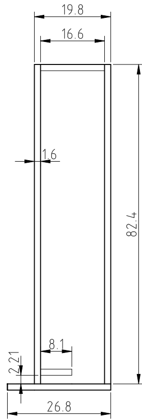
TABAQ W4-1337 HK V. 1.0 SIDE VIEW
