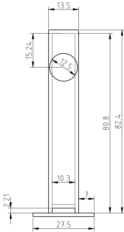
TABAQ W4-1337 HK V. 10 FRONT VIEW
